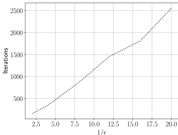
Figure 4. The results of Algorithm 1, for the problem 6.7.
