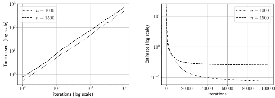
Figure 1. The results of Algorithm 4 for IEP with different values of n and m = 10 .
