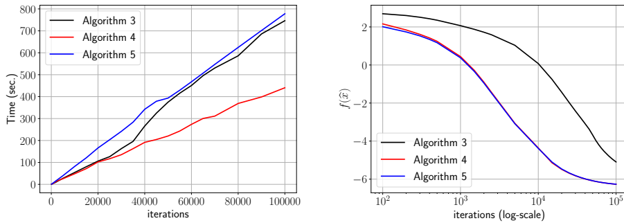
Figure 2. The results of Algorithms 3, 5 and 4 for IEP with n = 1000 and m = 10 .
